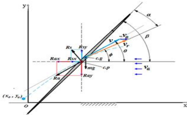
Fig.1 Javelin free body diagram.
